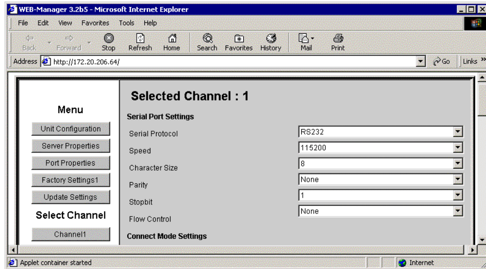
Figure 1-1. Lantronix Web-Manager
